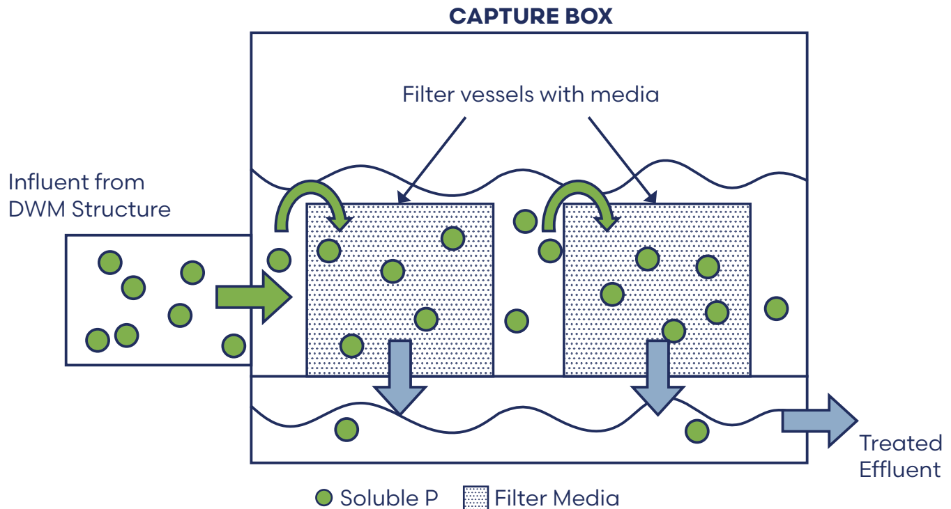
Figure 3. Illustration of phosphorus-laden water moving through a CAPTURE™ box.
