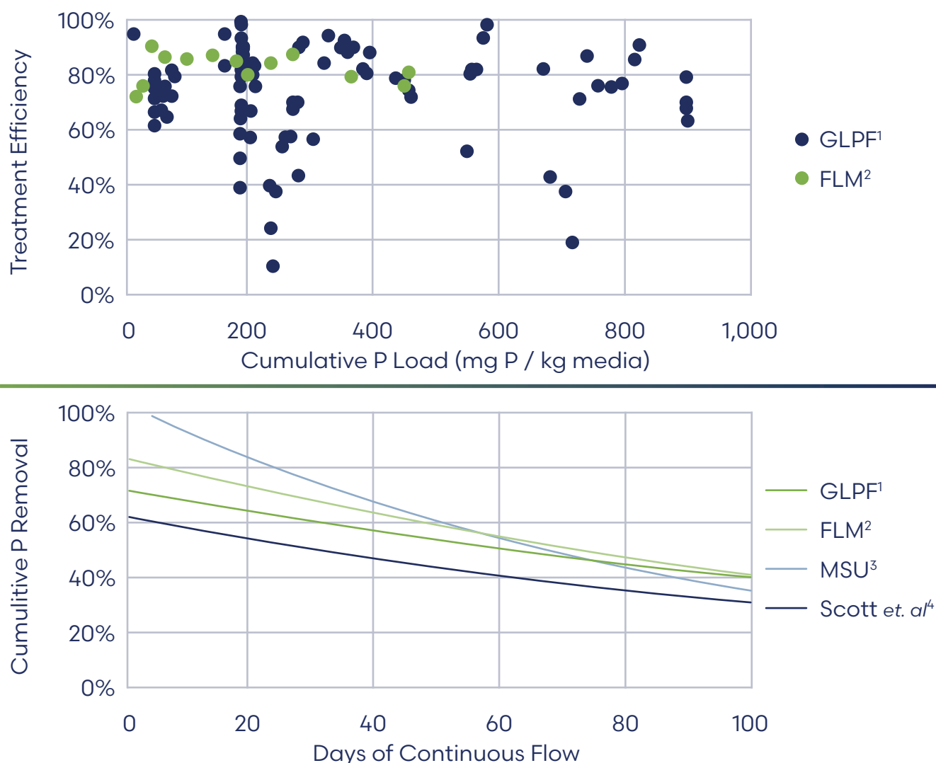
Figure 7. Field testing results (top) and extrapolated performance life (bottom). "Days of Continuous Flow" assumes a single CAPTURE™ box receiving an average 45 GPM constant flow containing 200 µg/L of soluble phosphorus.
